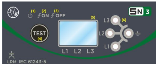
Fig. 2.3.1. Front panel view
